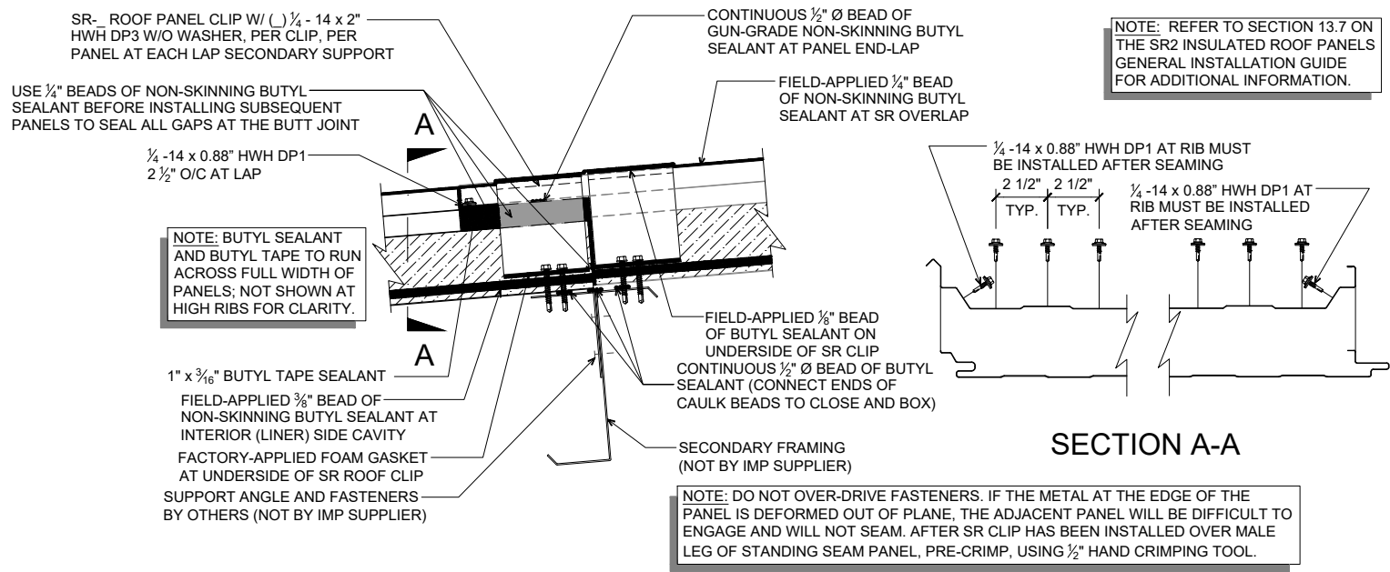
# SR ROOF PANEL NON-STAGGERED ENDLAP (SECTION VIEW)
